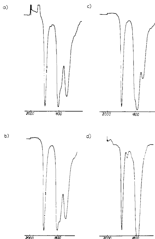
Figure 1. IR spectra of solutions formed upon addition of sequential amounts of \text{PPN}^+\text{Cl}^- to \text{Na}_2[(\eta^5\text{-C}_5\text{H}_5)\text{V}(\text{CO})_3\text{H}] in THF.
